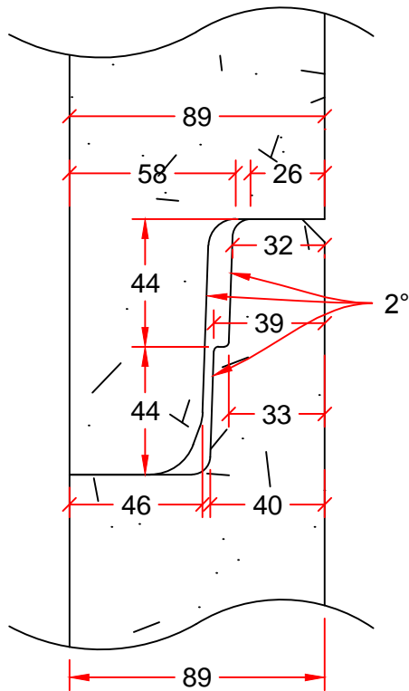
JOINT DETAIL
