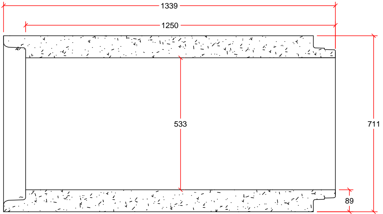
PIPE DETAIL
