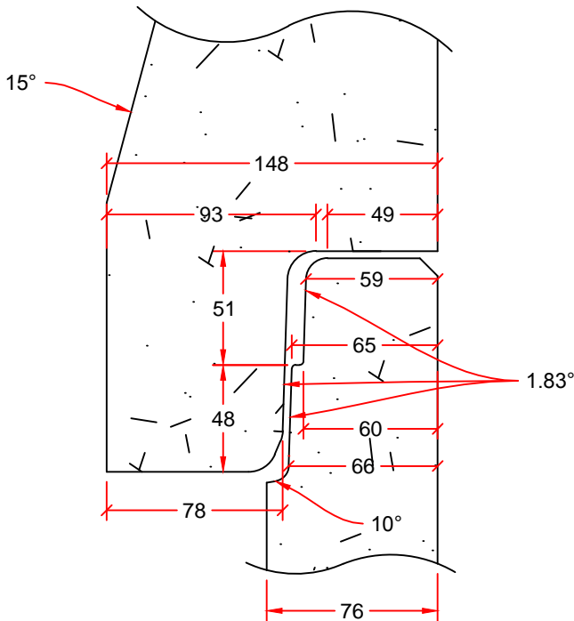
JOINT DETAIL
