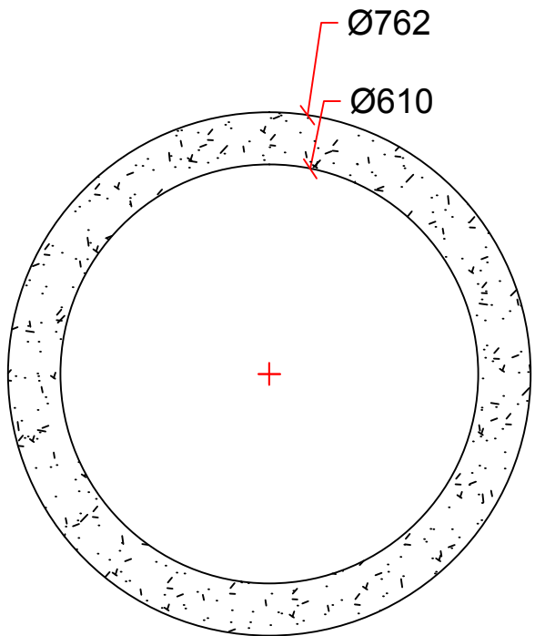
SECTION DETAIL
