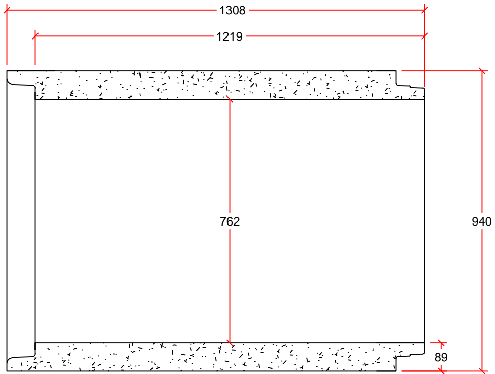
PIPE DETAIL
