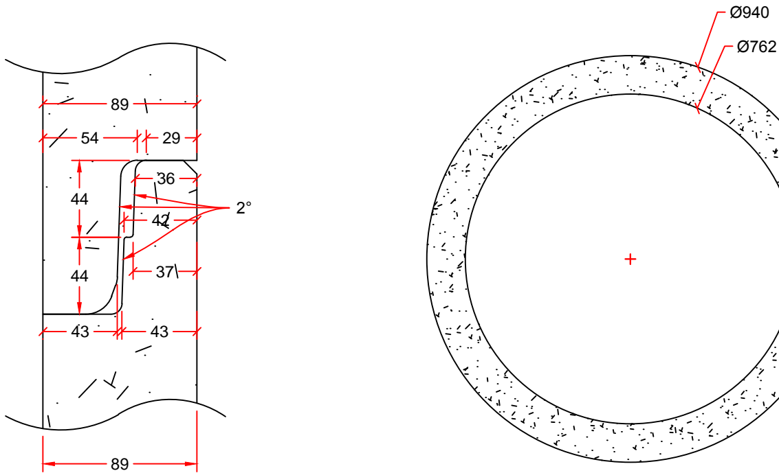
PIPE DETAIL
