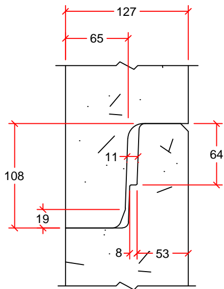
JOINT DETAIL
