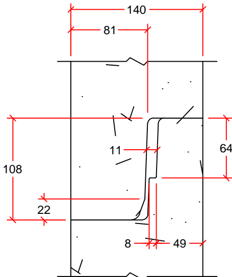
JOINT DETAIL
