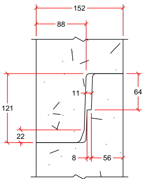
JOINT DETAIL
