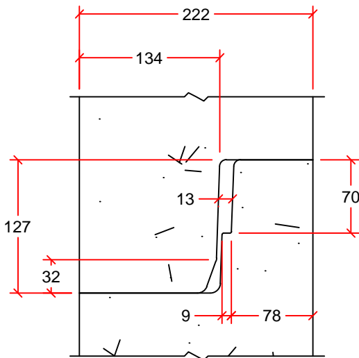
JOINT DETAIL
