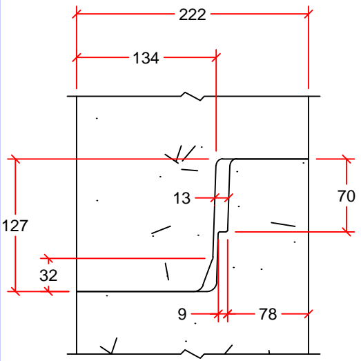
JOINT DETAIL
