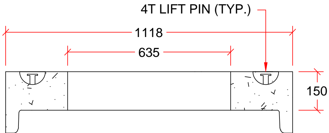
900mm SLAB TOP W/ 635mm ROUND OPENING
