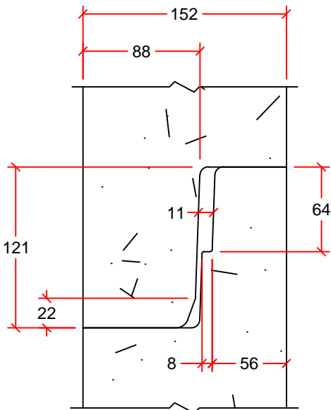
JOINT DETAIL
