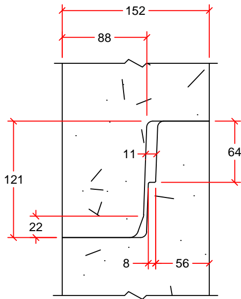
JOINT DETAIL
