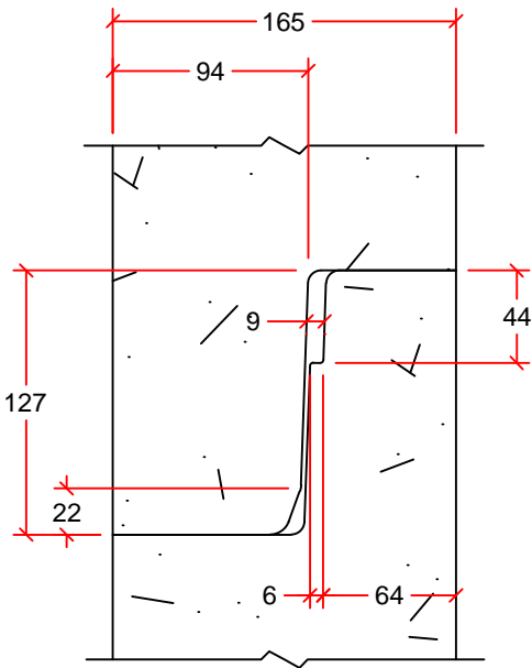
JOINT DETAIL
