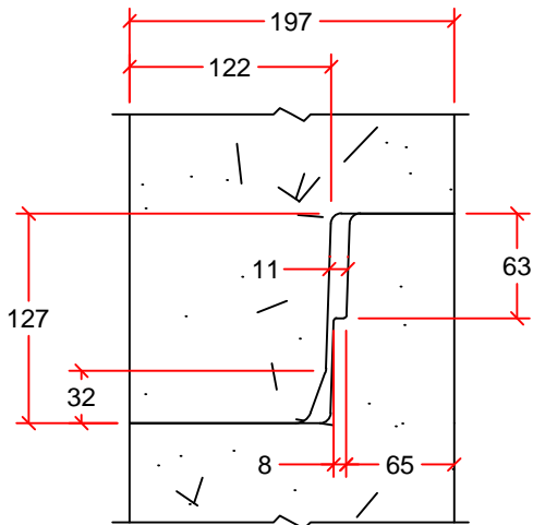
JOINT DETAIL
