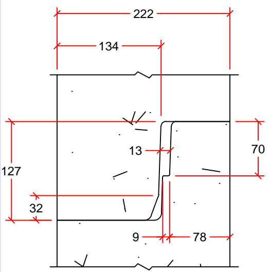
JOINT DETAIL
