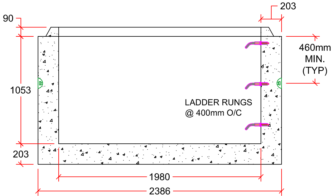
SIDE VIEW
